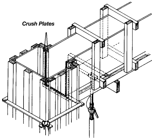
Figure 192 — Crush Plates
