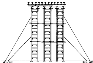
Figure 205 High Guyed Towers
