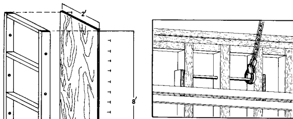
Figure 192 — Crush Plates
